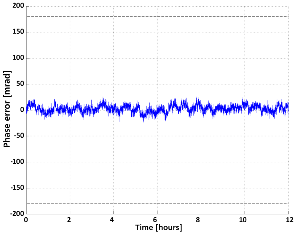
Figure 8: APUASYN20 typical time domain channel-to-channel phase error at 10 GHz - measured over 12 hours
