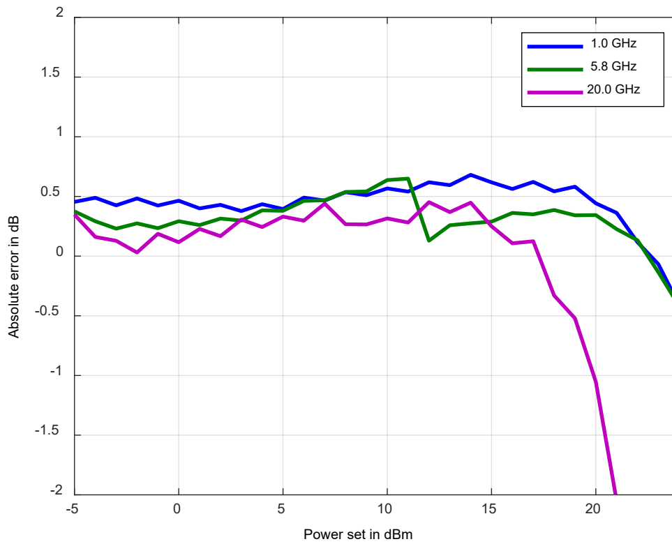
Figure 4: Power linearity
