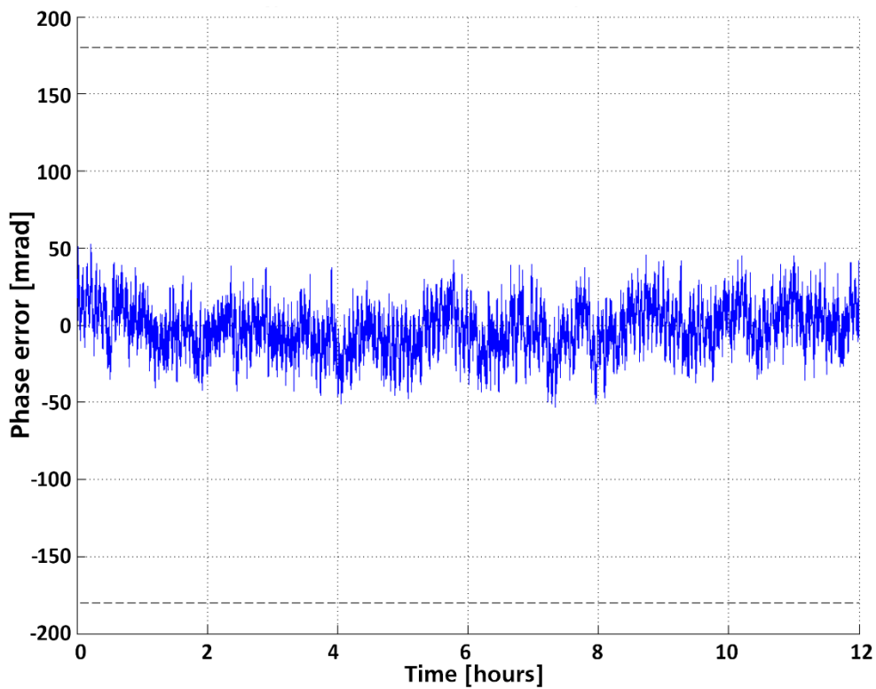
Figure 9: APUASYN20 typical time domain channel-to-channel phase error at 20 GHz - measured over 12 hours
