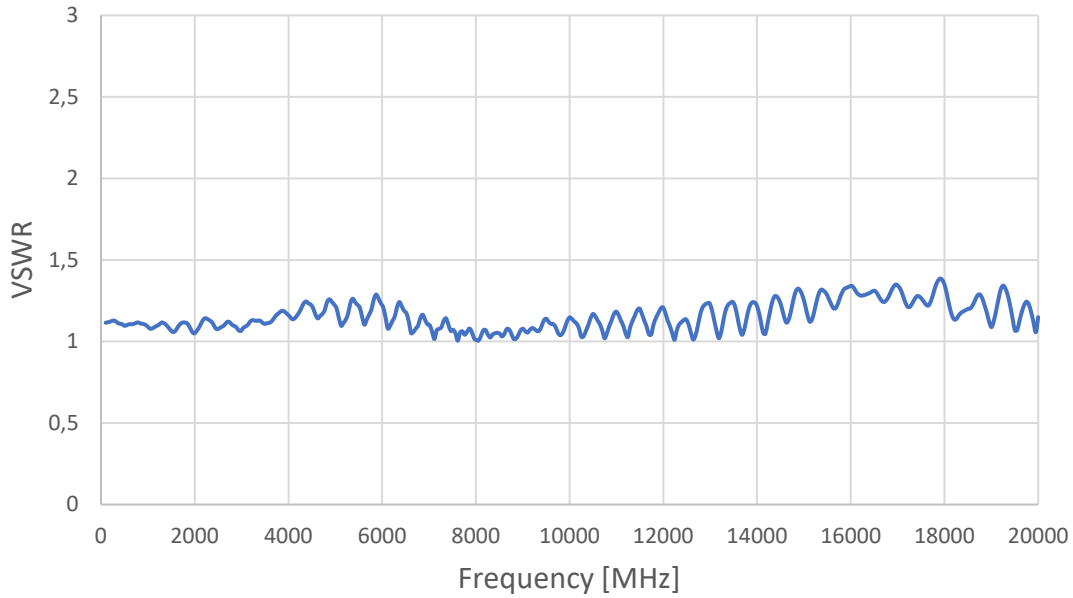
Figure 10: Typical VSWR (APULN20)
