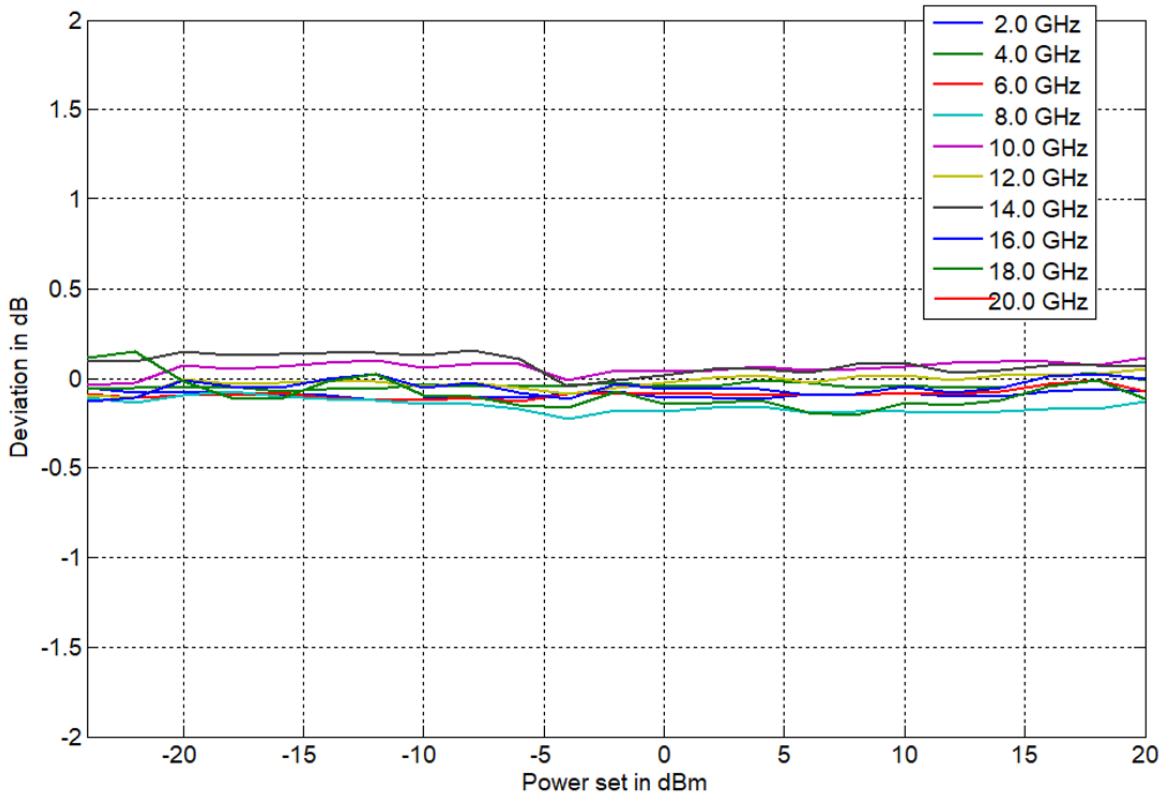
Figure 12: Typical Output Power Linearity (APULN20)
