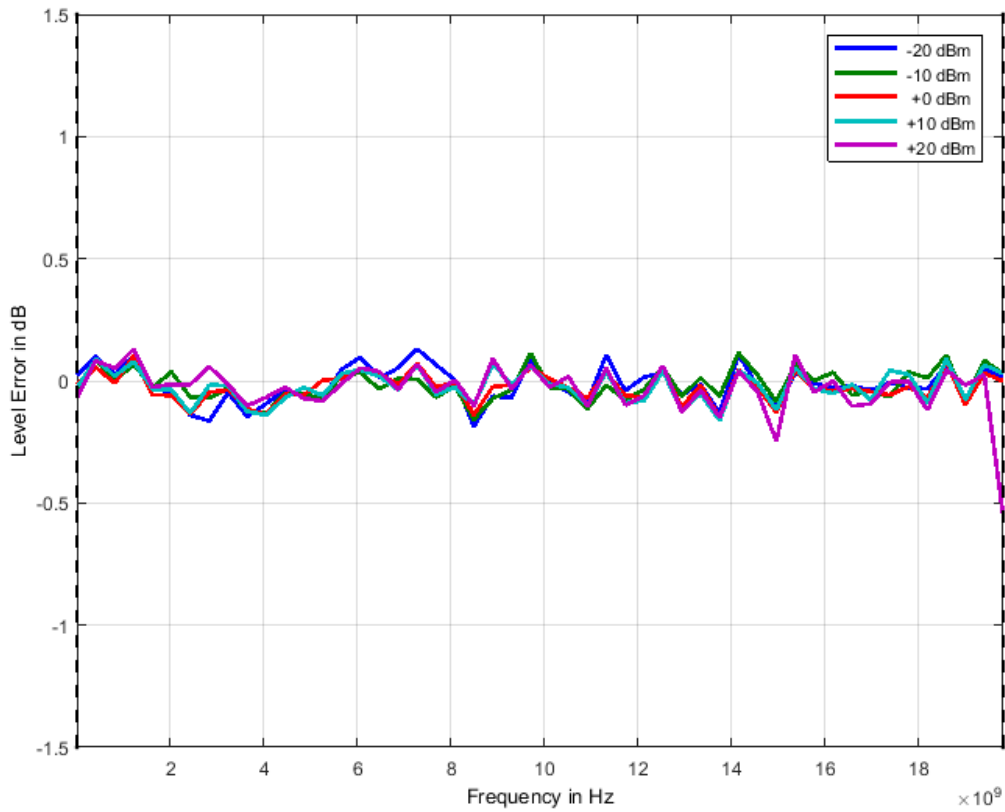
Figure 11: Typical Frequency Response 0 to 20 GHz at different power levels (APULN20)
