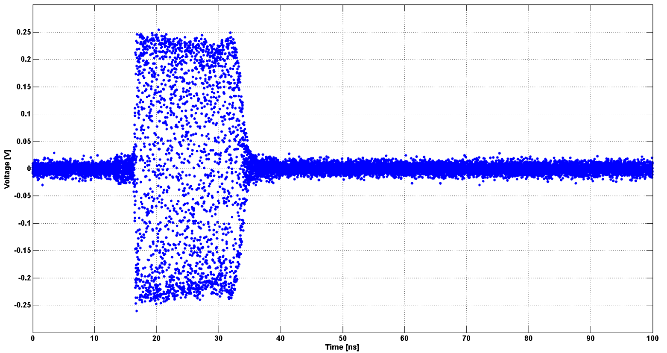
Figure 15: APULN40 option FS Pulse Modulation 20 ns - 40 GHz Carrier Frequency
