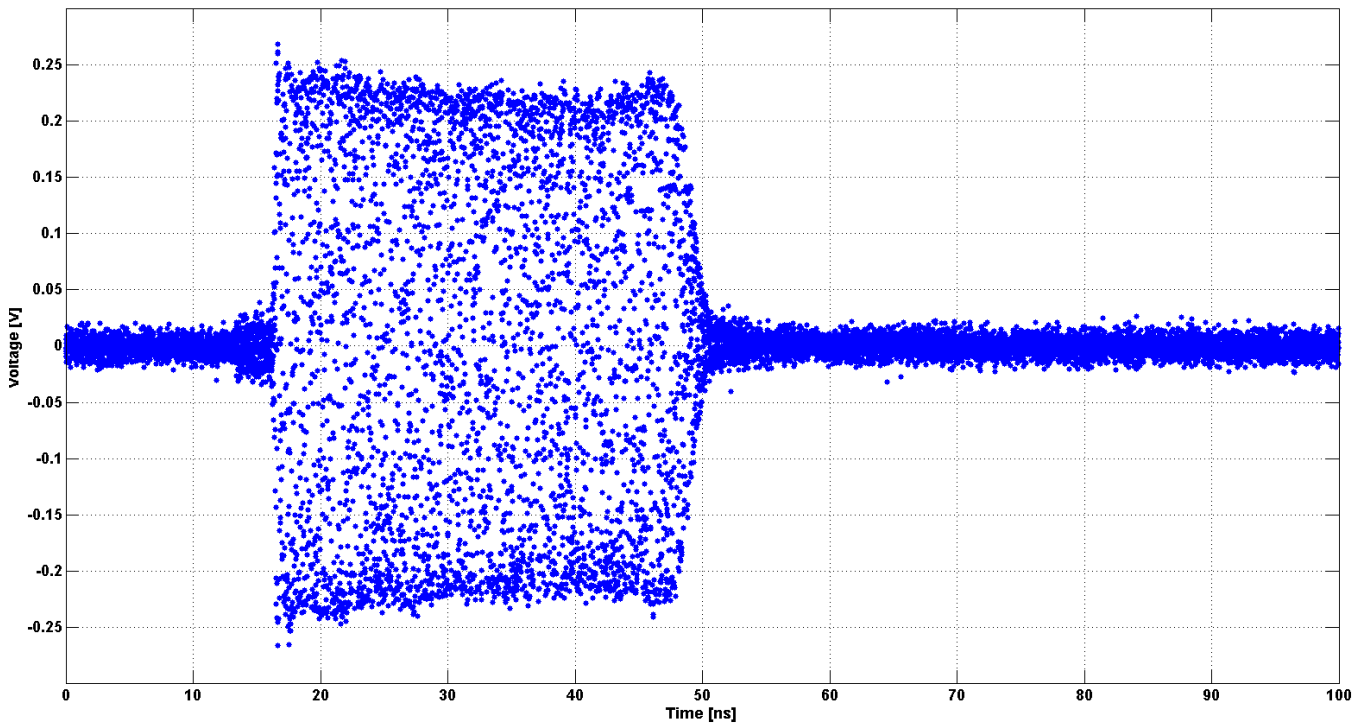
Figure 14: APULN40 option NP or NEC Pulse Modulation 30 ns - 40 GHz Carrier Frequency
